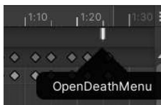
Slika 12. Animation event
